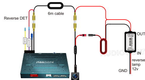
(Rectifier version)
